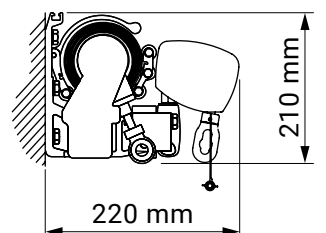
wall installation
