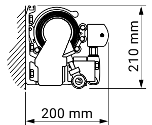
wall installation
