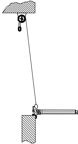
Installation to the arm hook (arm horizontal)
