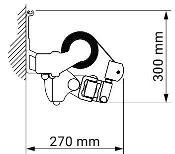
wall installation
